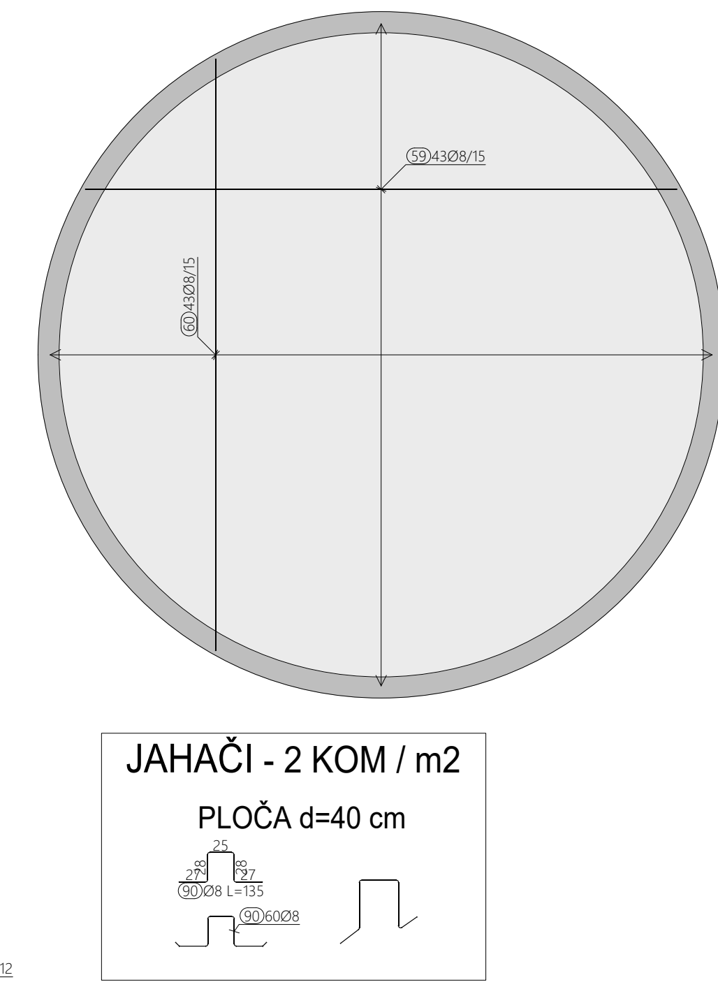
ARMATURA GORNJE ZONE BAZENA, M 1:50
