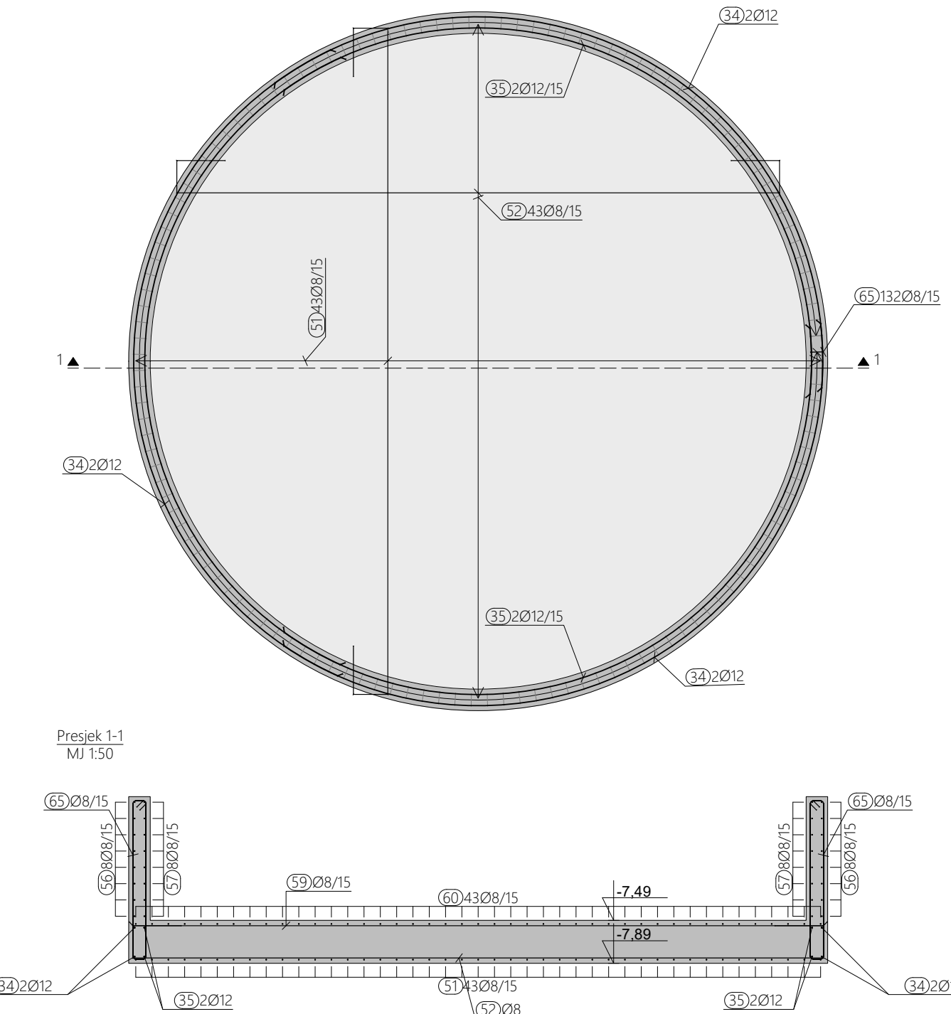
ARMATURA DONJE ZONE I ANKERI BAZENA, M 1:50
